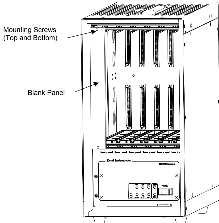
Figure 2-2, Blanking Panels
