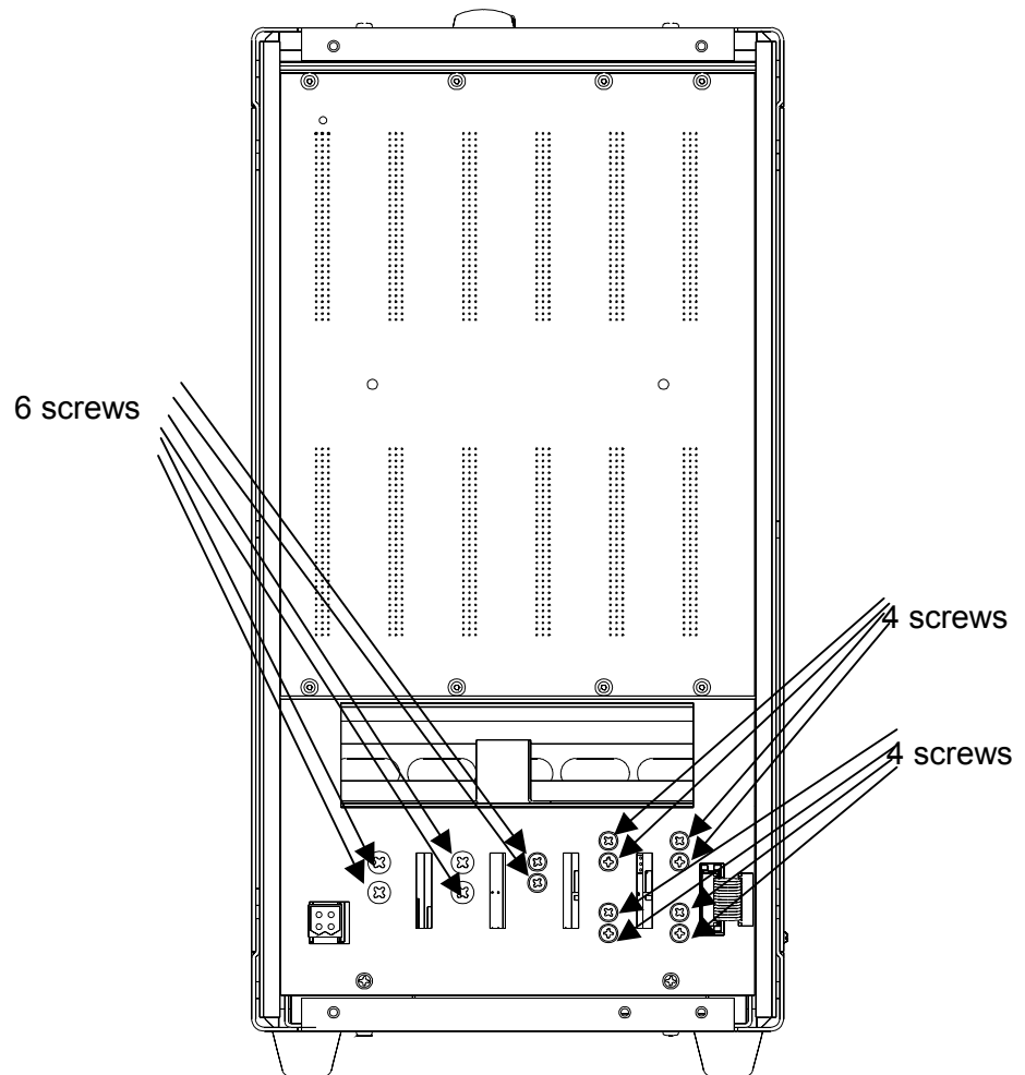
Figure 5-4, Loosening The 14 Screws.
