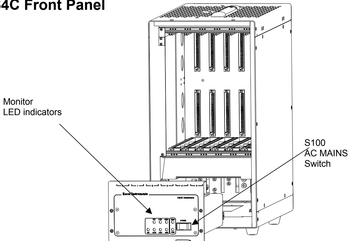
Figure 3-1, 1264C Front View
