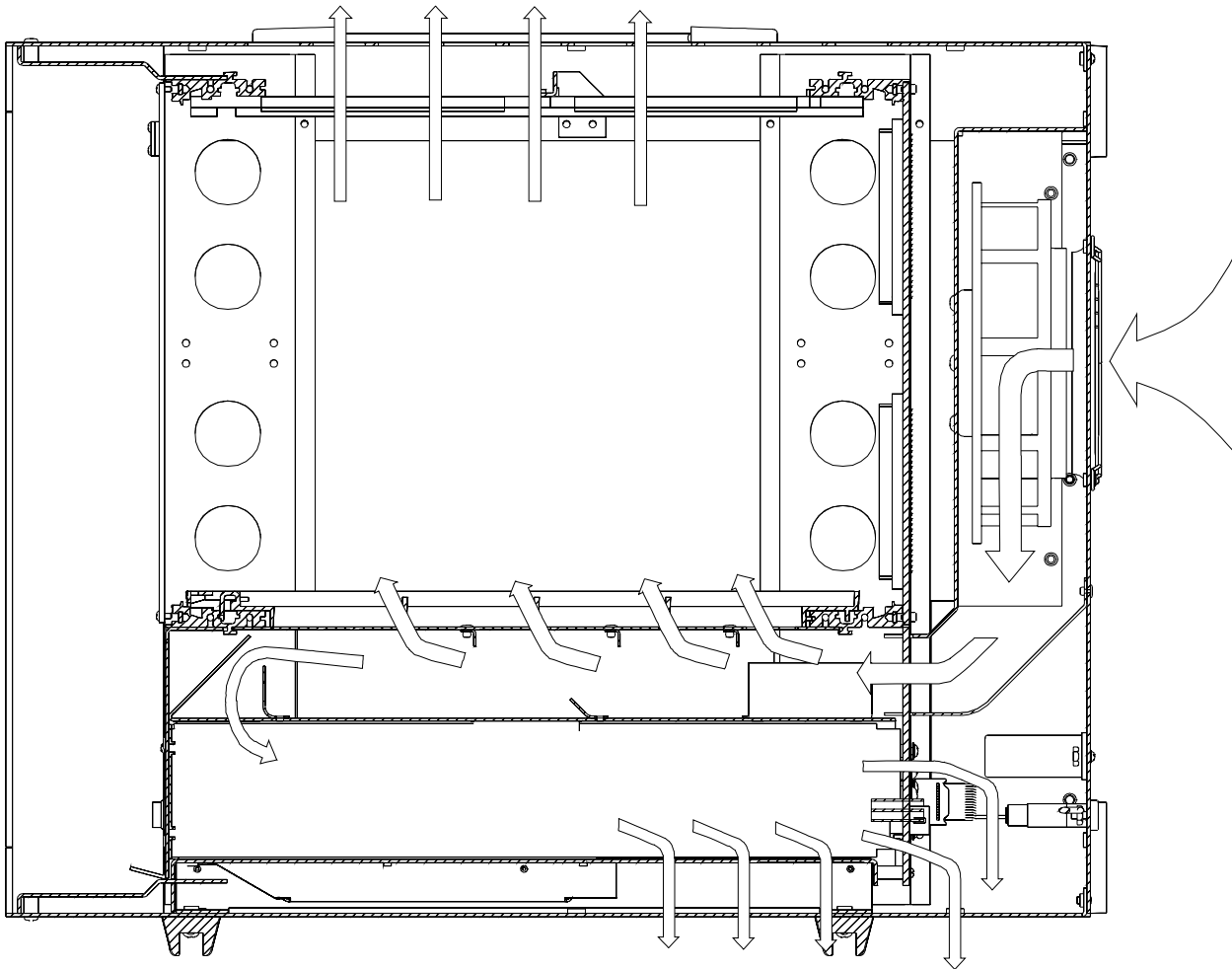
Figure 1-5, 1264C Positive Pressure Cooling System.
