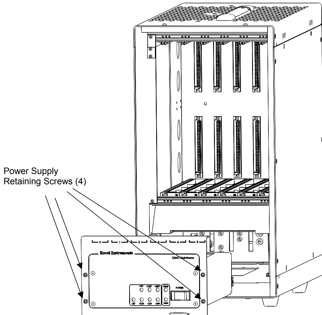
Figure 5-3, Removing The Power Supply
